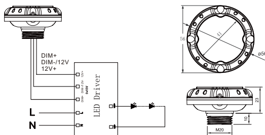
Wiring diagram
