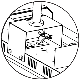
WSD-LHB-PMK-LID Pendant Mounting Box
