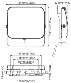
90W&120W(Yoke Mount)
