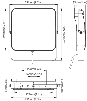
40W&65W(Trunnion Mount)
