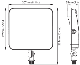
40W&65W(Knuckle Mount)
