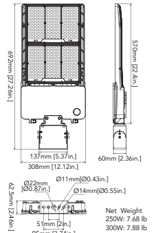
250W/300W (Yoke Mount)
