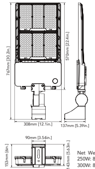
250W/300W (Adjustable Square Mount)
