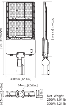
250W/300W (Slipfitter Mount)
