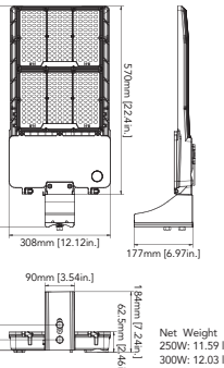
250W/300W (Pole Mount)
