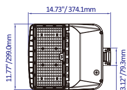
150WS Without Mounting Bracket
